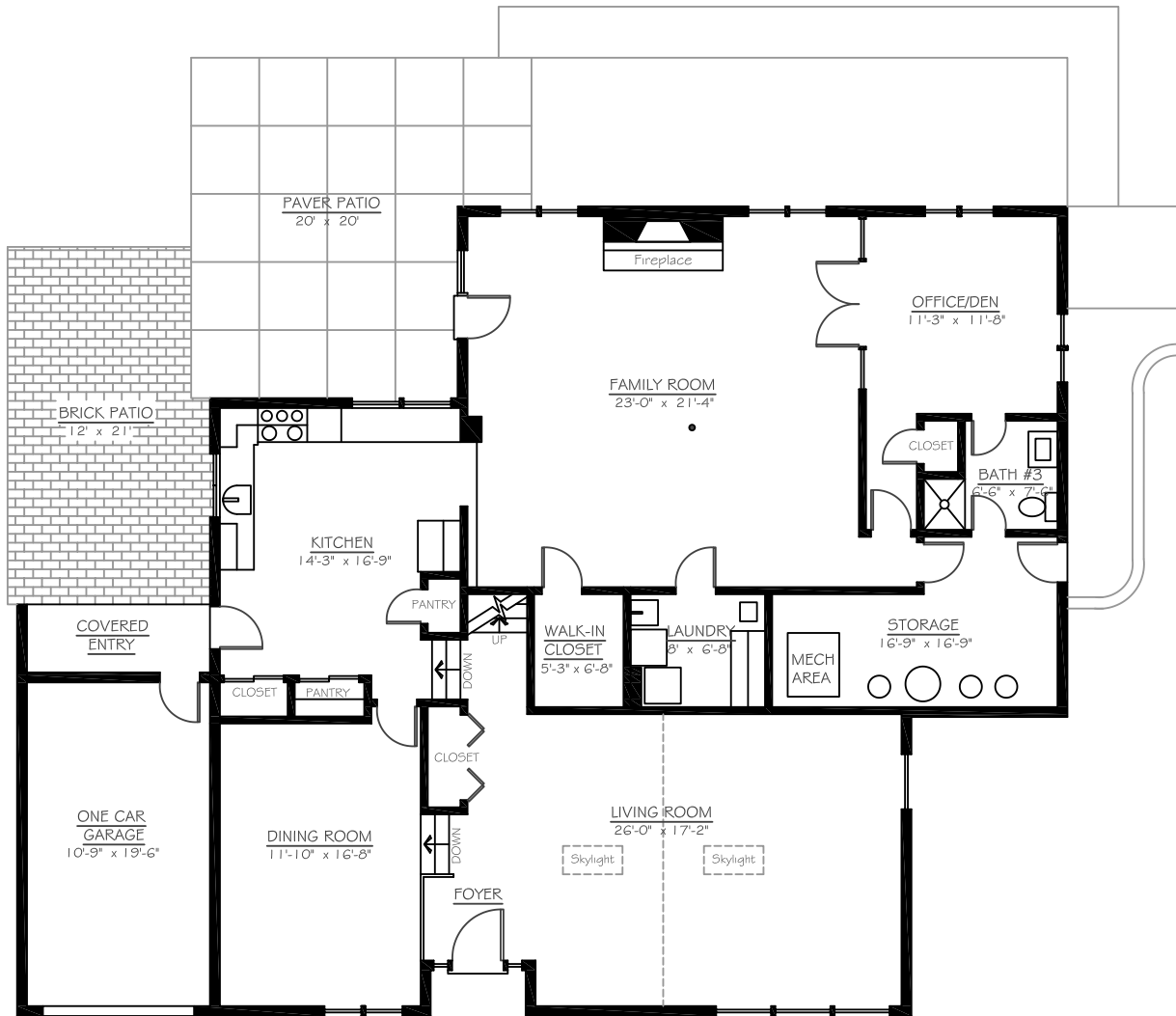
MAIN LEVEL
