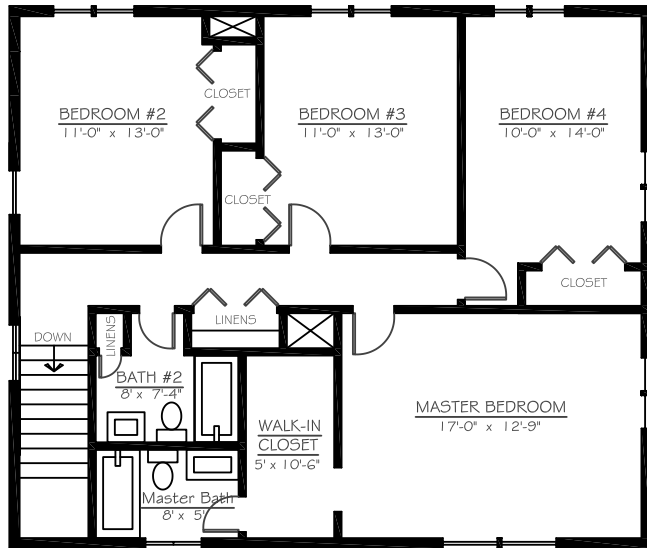
UPPER LEVEL
