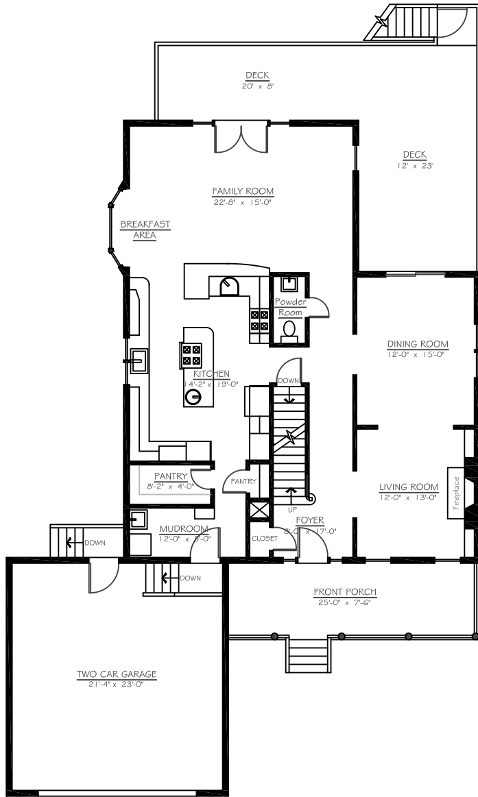
MAIN LEVEL
