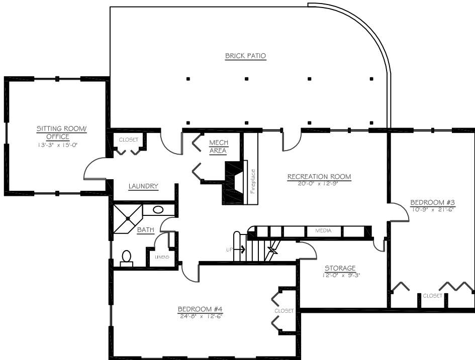
LOWER LEVEL
