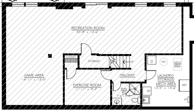
LOWER LEVEL Finished Square Footage = 1168 (Includes Wall Thickness)
