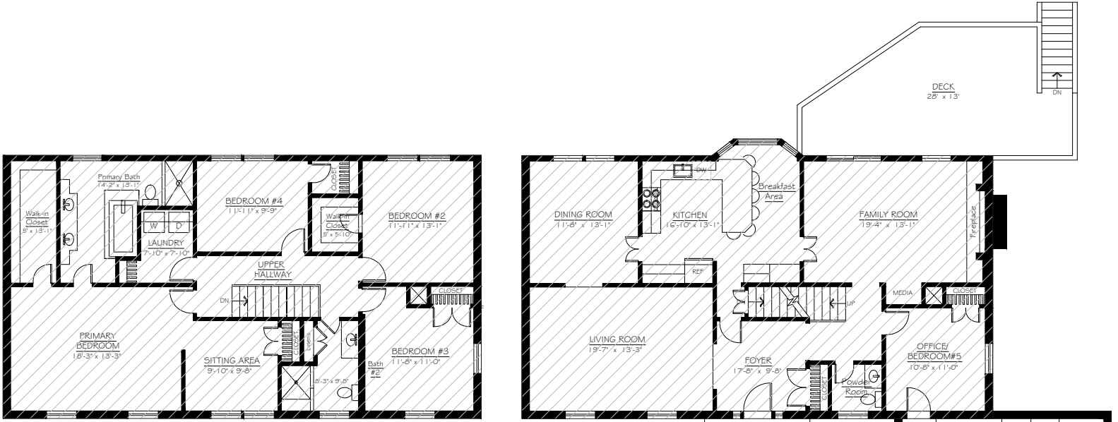
UPPER LEVEL Finished Square Footage = 1431 (Includes Wall Thickness)
