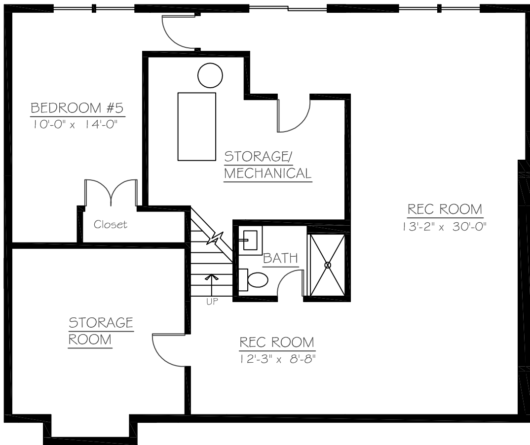
LOWER LEVEL
